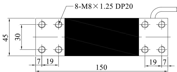
俯視(Top View)
