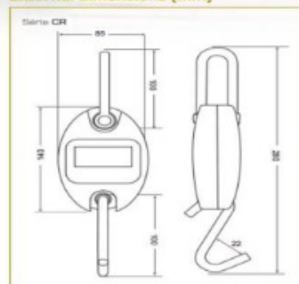
External dimensions (mm)
